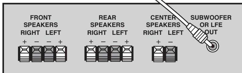
Back of Audio Receiver
